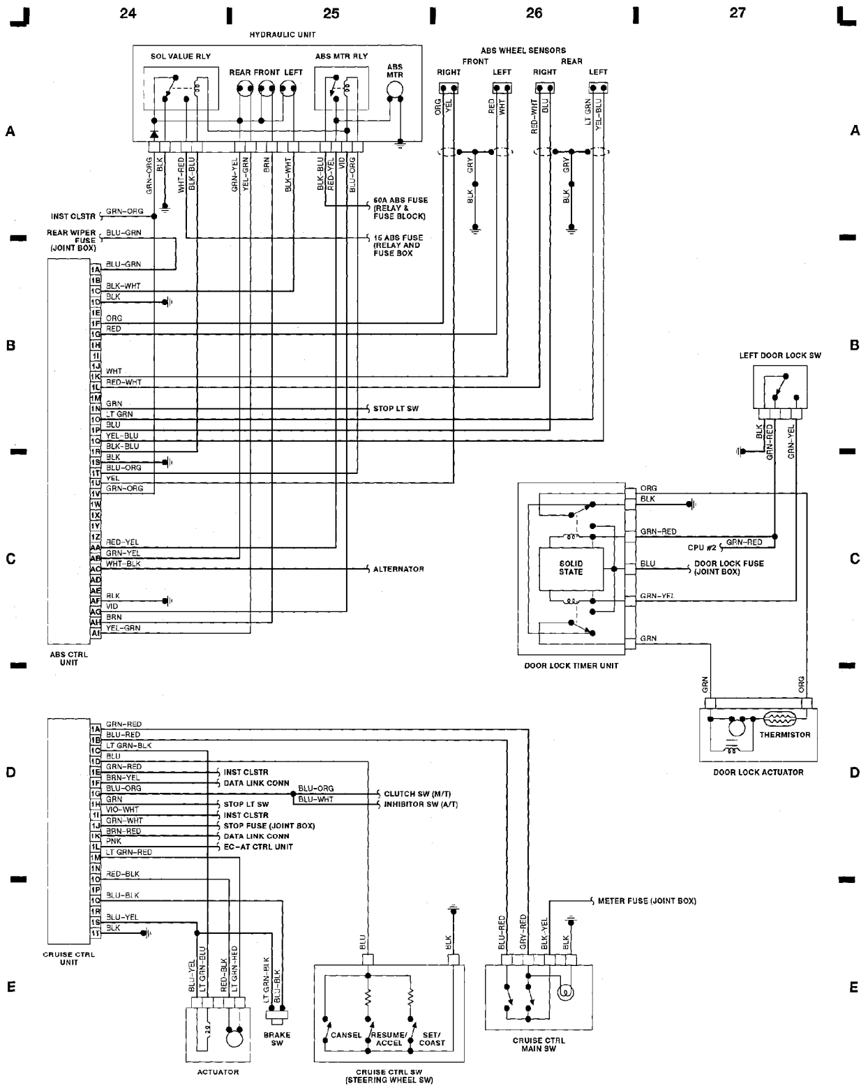
Fig. 7: Cruise Ctrl Unit, Hydraulic Unit (Grids 24-27)
