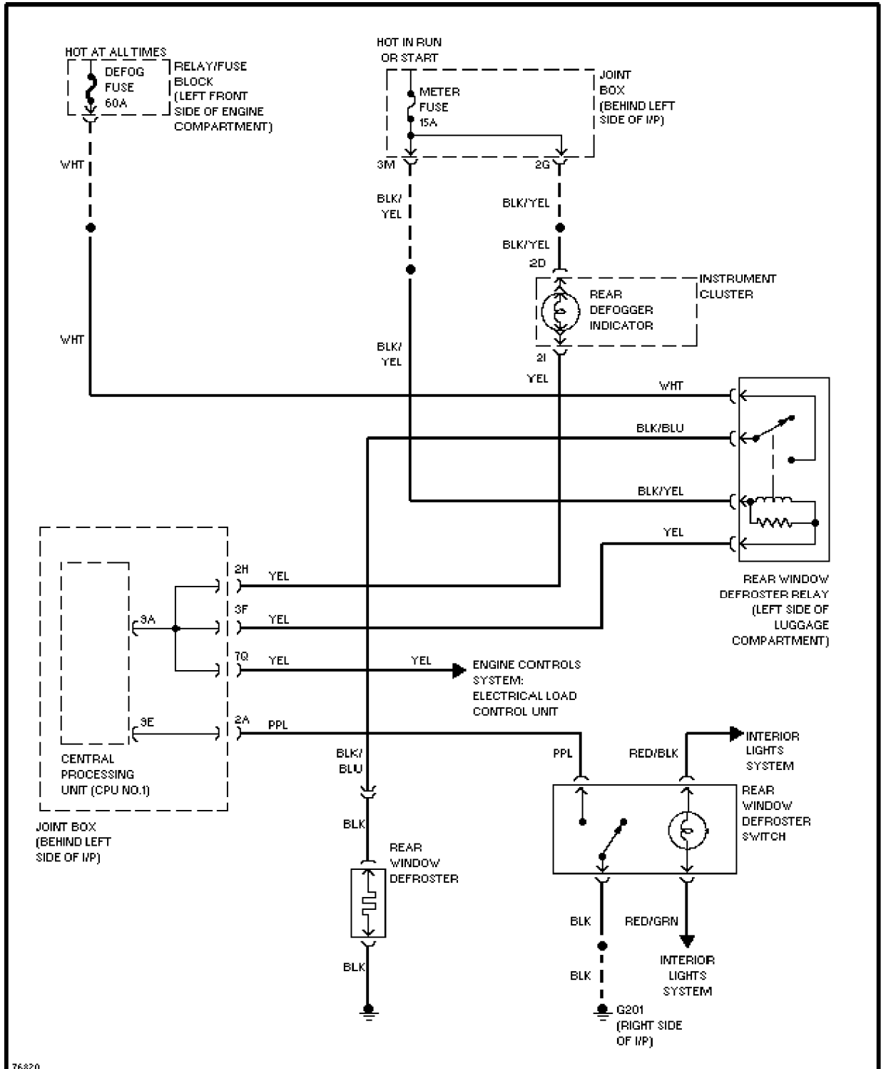
Defogger Circuit
