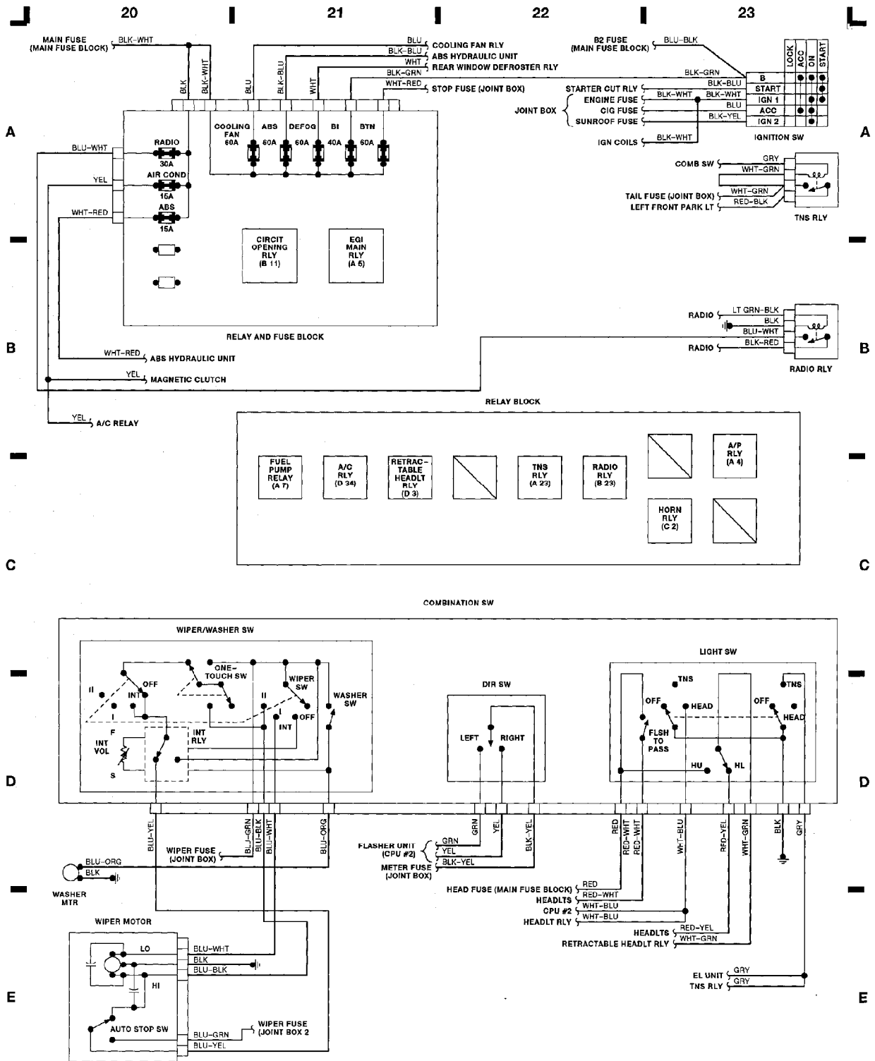
Fig. 6: 94F30754 20 21 22 23 Combination Sw, Wiper/Washer Sw (Grids 20-23)
