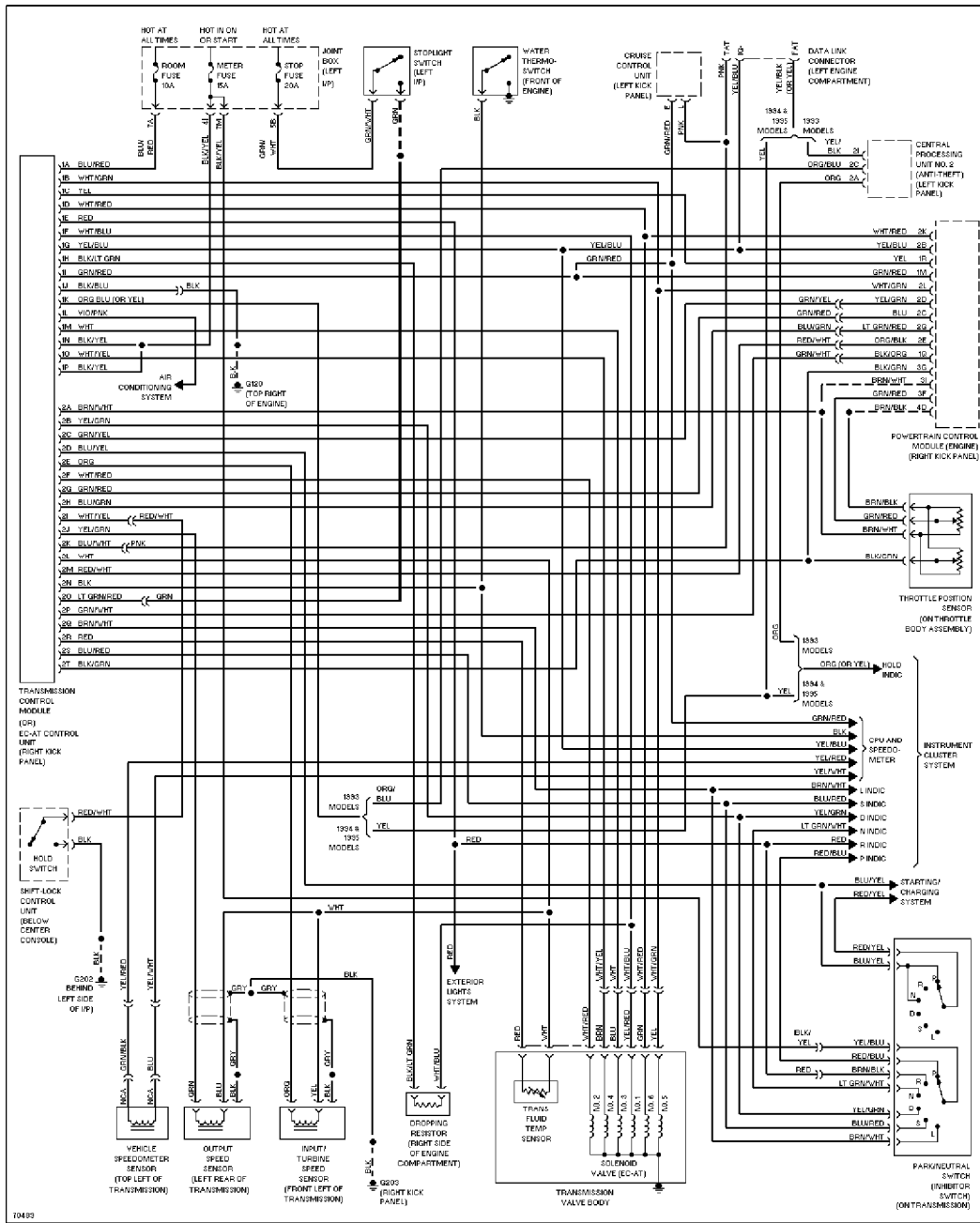
Transmission Circuit
