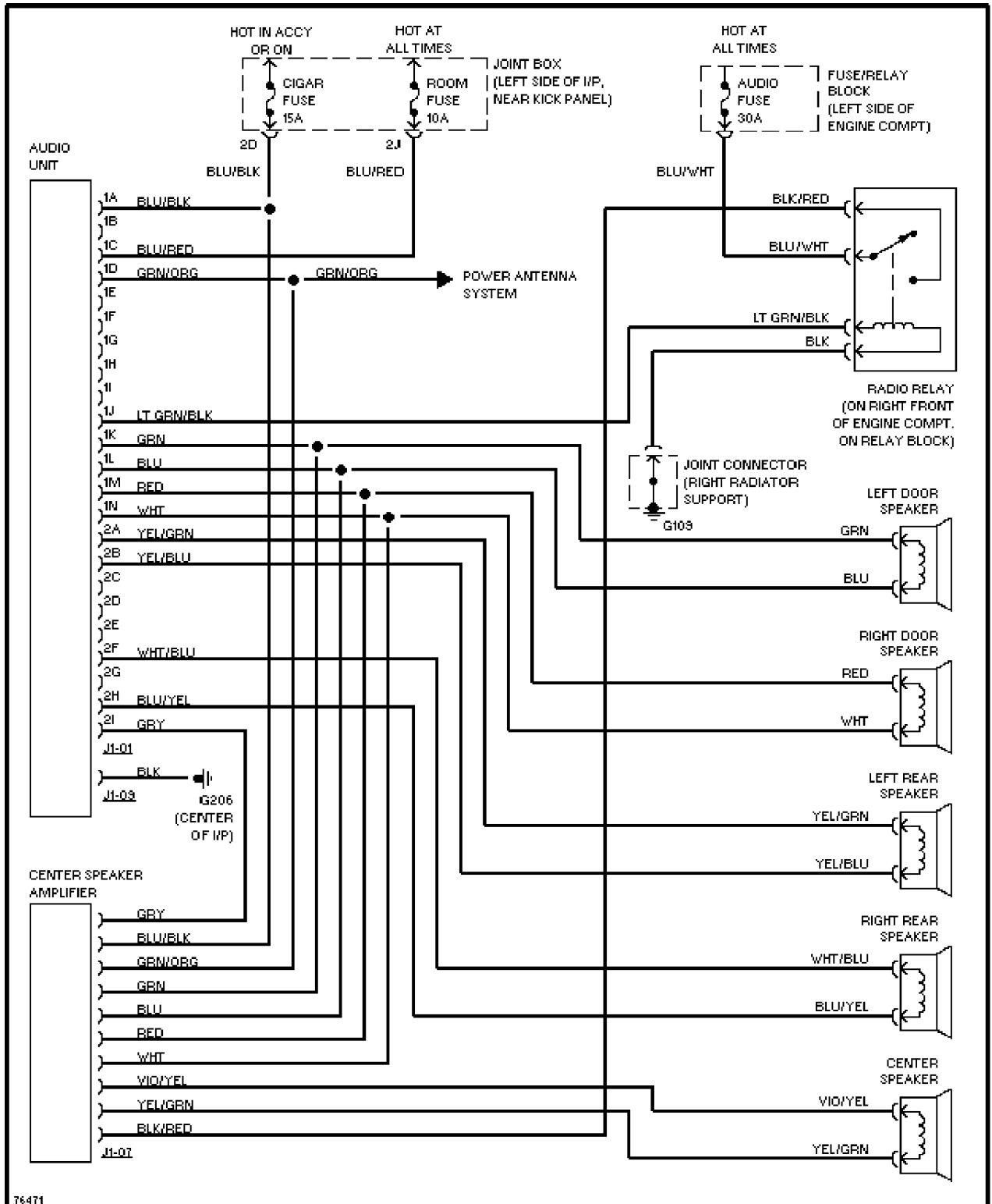
Radio Circuits, W/O Bose Acoustic Wave System
