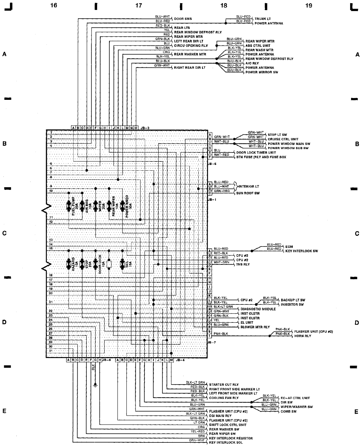
Fig. 5: Joint Box (Cont.) (Grids 16-19)
