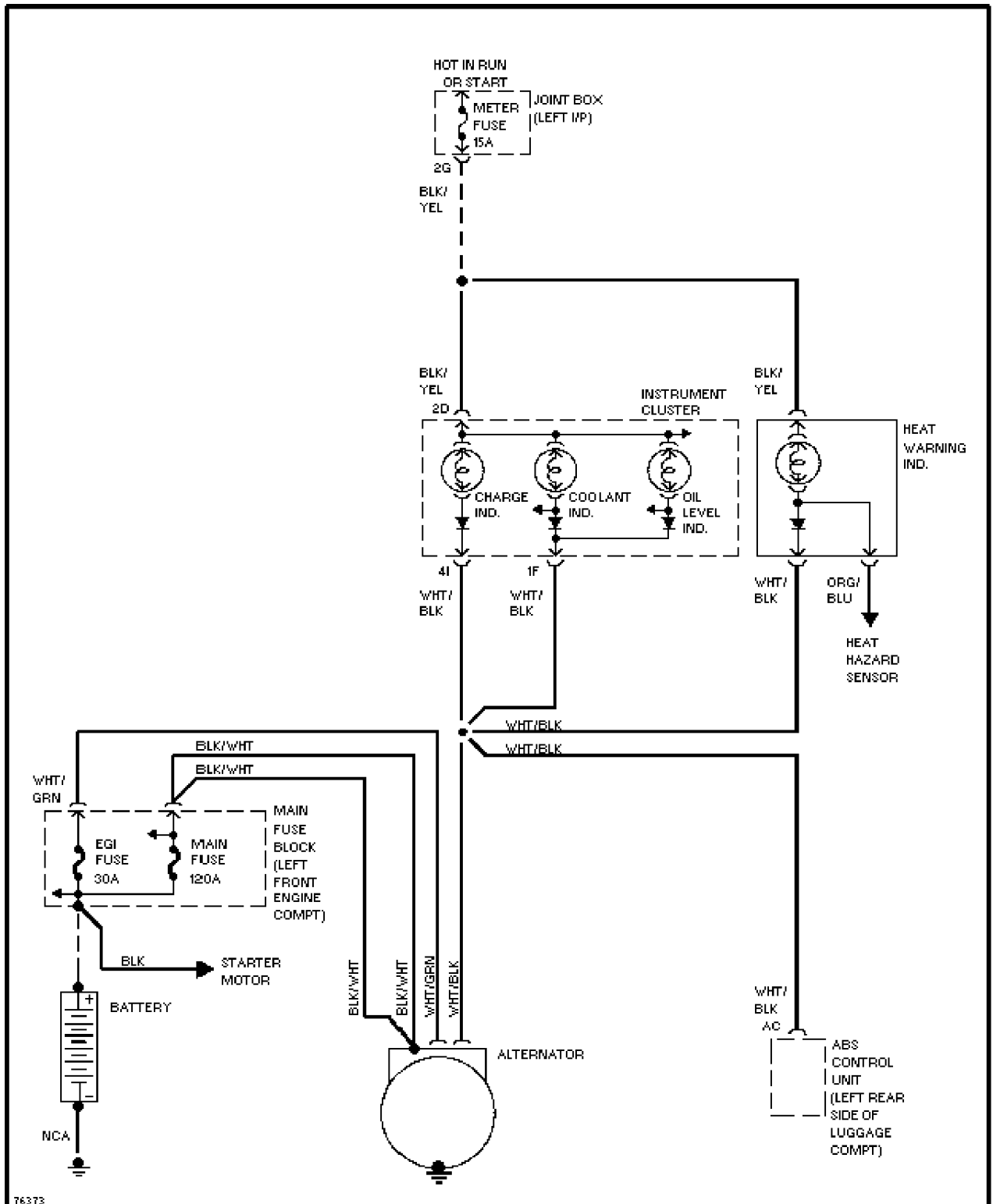
Charging Circuit
