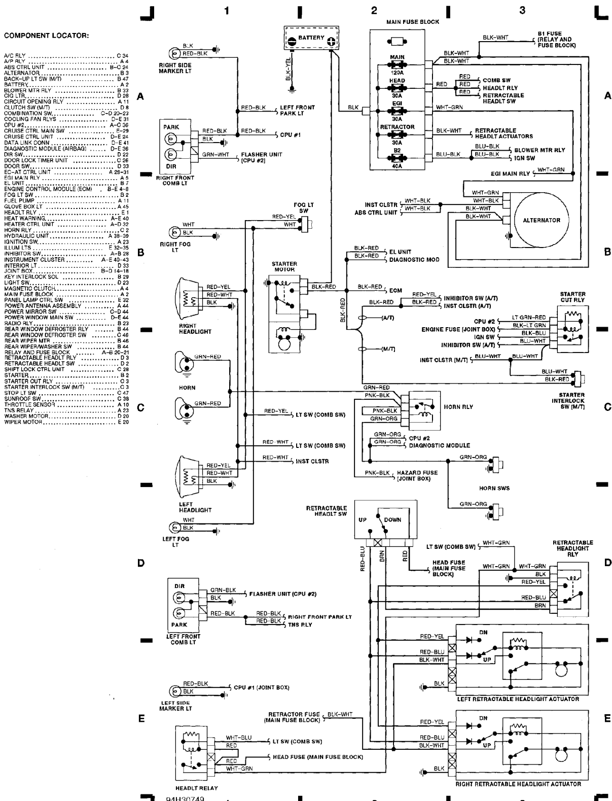
Fig. 1: Engine Compartment & Headlights (Grids 1-3)
