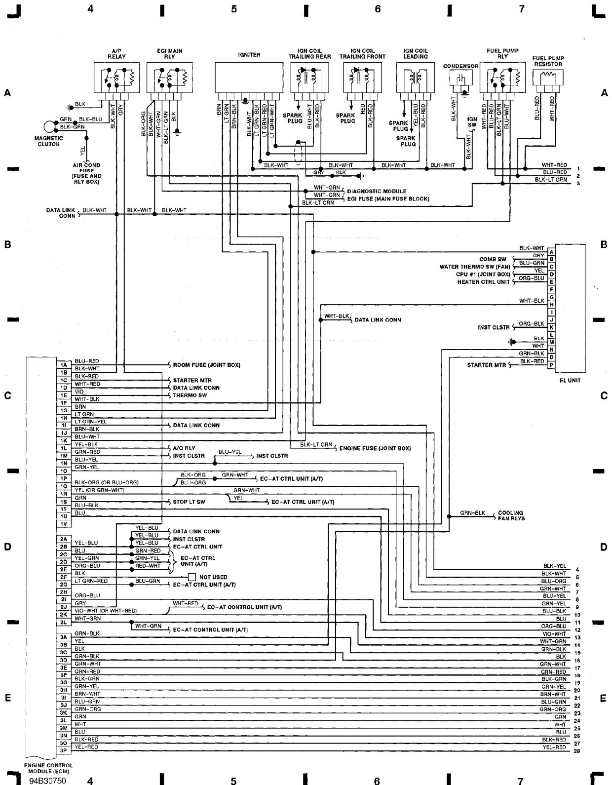
Fig. 2: Engine Ctrl Mdl, EL Unit, Fuel Pump Rly (Grids 4-7)
