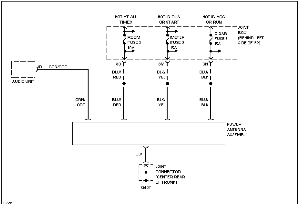
66591 Power Antenna Circuit
